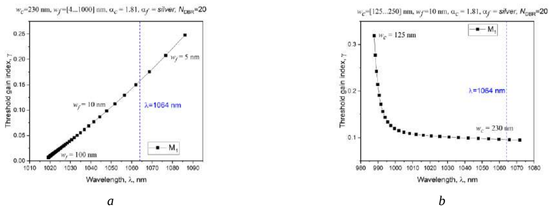
Fig. 4. Trajectories of the modes M_1 of the active microcavity covered with silver film and lying on 20-pairs DBR under the variation of the silver film thickness w_f from 4 to 1000 nm (a) and active layer thickness w_c from 125 to 250 nm (b)
